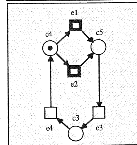
Figure 4: The couple of events which let the net be non-simple
