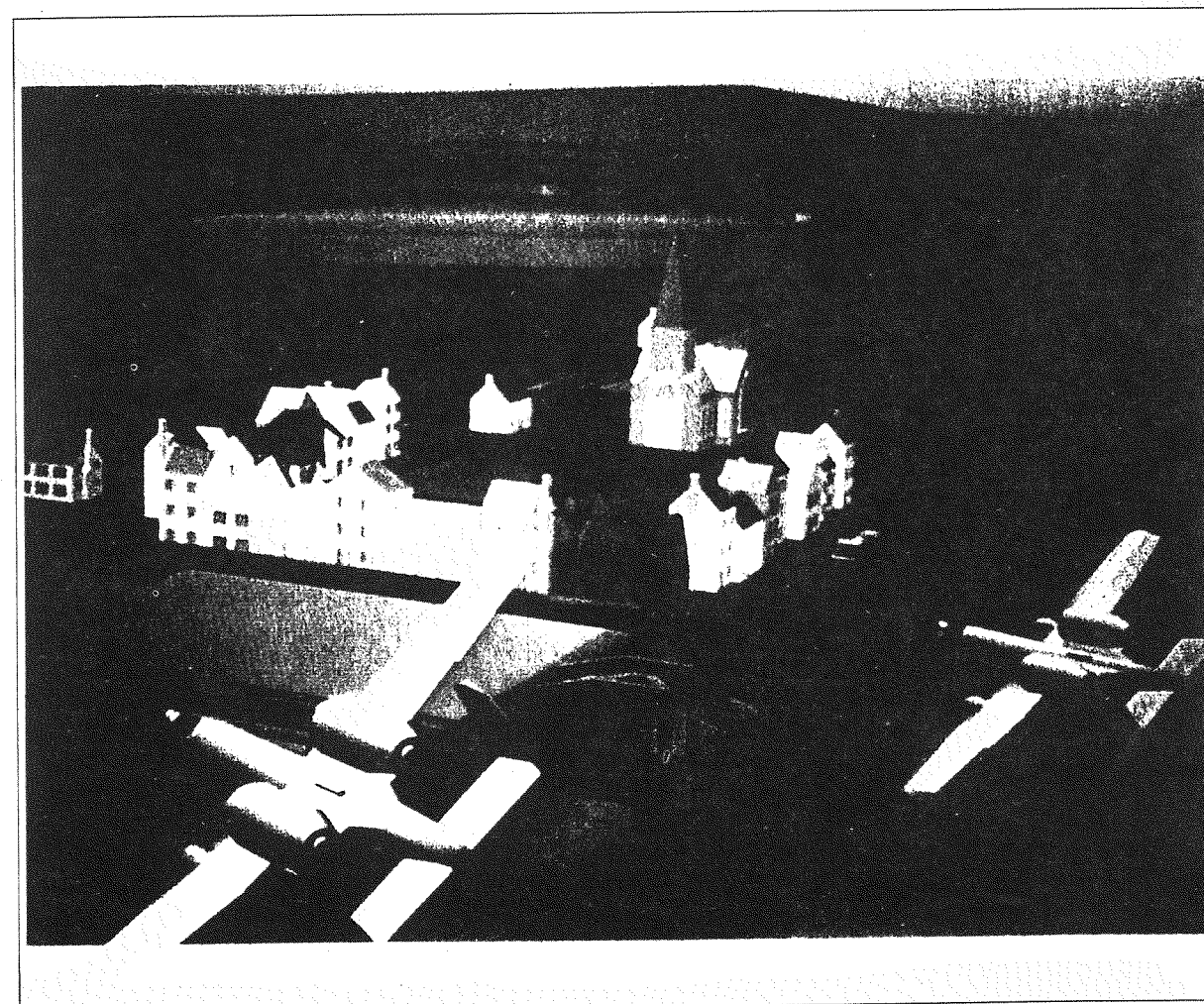
Figure 1: Evans & Sutherland CT5-A Simulator
