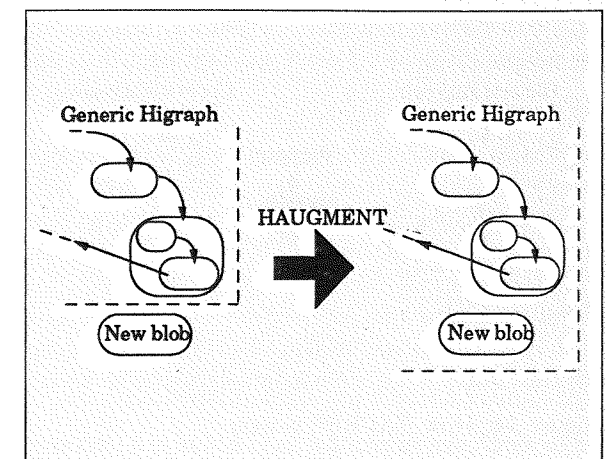
Figure 13: How HAUGMENT works.
