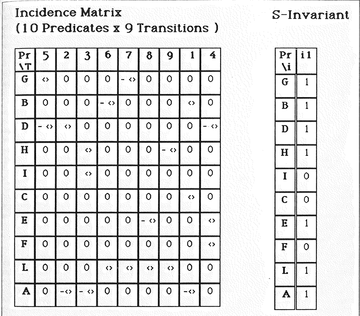
Figure 6: This figure shows the incidence matrix and an S-invariant
