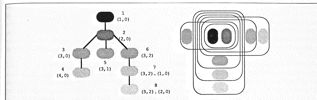
Figure 4: A delta tree of a document and the corresponding higraph: higher numbers gives chronological order of the insertions, and lower numbers give the address of the tree nodes for the system.
