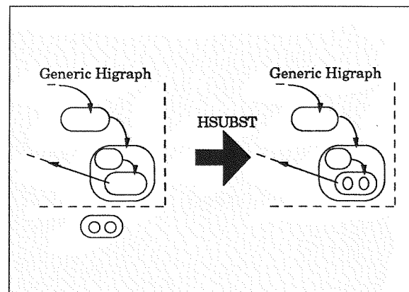
Figure 14: How HSUBST works.
