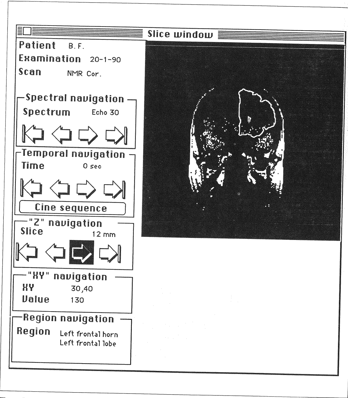
Figure 5: The slice window. The areas on the left correspond to the different possibilities of navigation in in spectra, times and Z coordinates. XY navigation gives the cursor coordinates over the image and "Region navigation" gives the name of the region (or regions) touched by the cursor. In this figure The cursor is over the frontal horn of the left lateral ventricle, and is inside a wider area corresponding to the left frontal lobe of the brain. Both the frontal horn contour and the left frontal lobe contour are enhanced
