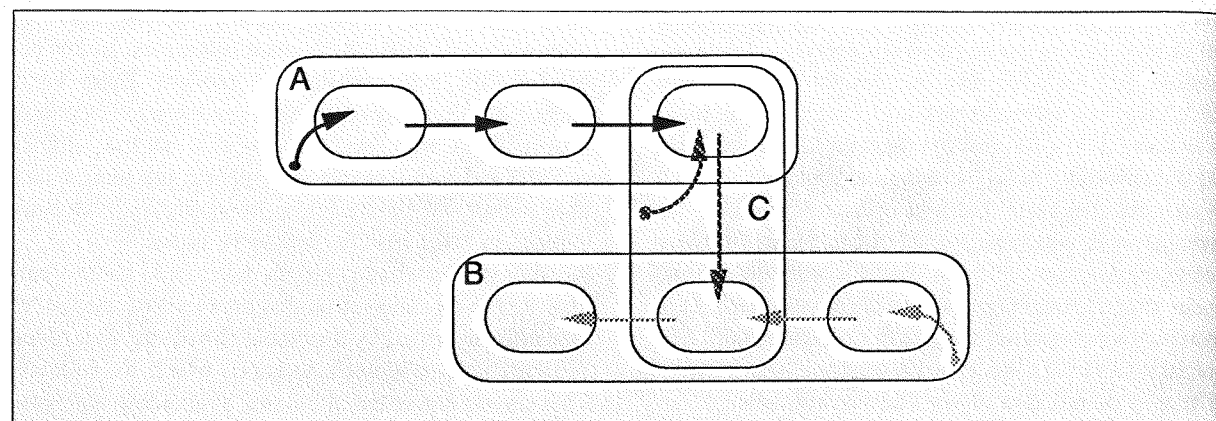
Figure 3: A simple s-higraph. Do note that every blob has its (first generation) subblobs structured in a chain.
