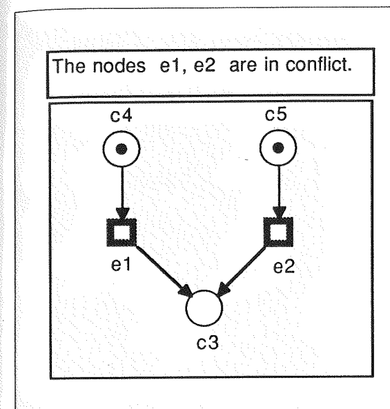
Figure 7: The highlighted events are in conflict
