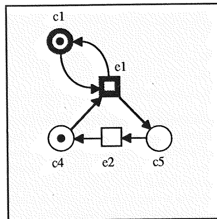
Figure 3: The couple of nodes which let the net be non-pure
