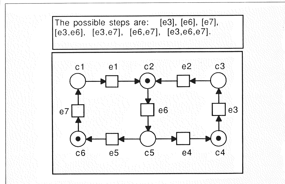
Figure 9: Show the possible steps which can occur in the current case of net
