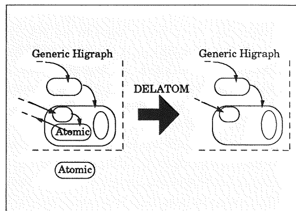
Figure 15: How DELATOM works.
